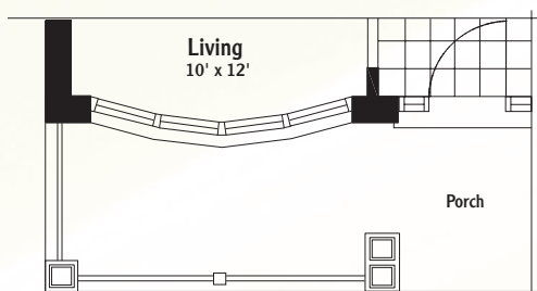
Partial Ground Floor Plan (Elevation B)
